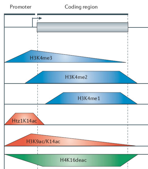
Figure 3 | Gradients of histone methylation and acetylation in active genes. A schematic representation of an active euchromatic gene is shown, with the promoter and coding regions indicated. The extent of modification at H3K4, H3K9, H3K14, H4K16 and Htz1K14 are shown. The level of modification is depicted by the height of the coloured shape. H3K4me3 is most enriched at the 5' end of active genes, whereas H3K4me2 and H3K4me1 are found in increasing amounts at the 3' end of the coding region. Acetylation of Htz1K14 is found at promoters, whereas acetylation detected by antibodies to H3 diacetylated at K9 and K14 peaks at the 5' end of genes. H4K16 is deacetylated at active genes and promoters.
